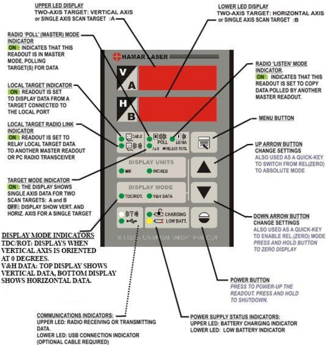
Figure 8 – R-1307+R Readout Control Panel Features
