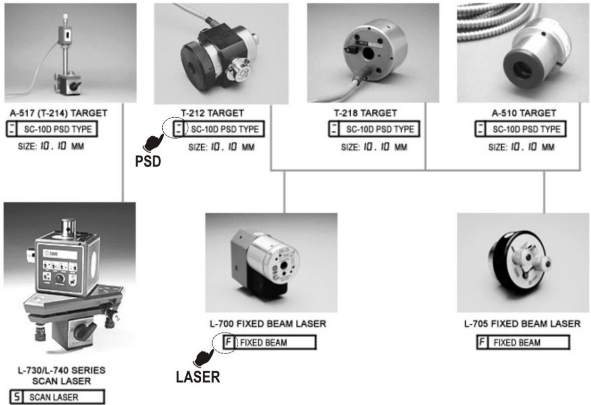
Figure 17 – Target PSD Descriptor, Standard Targets and Lasers
