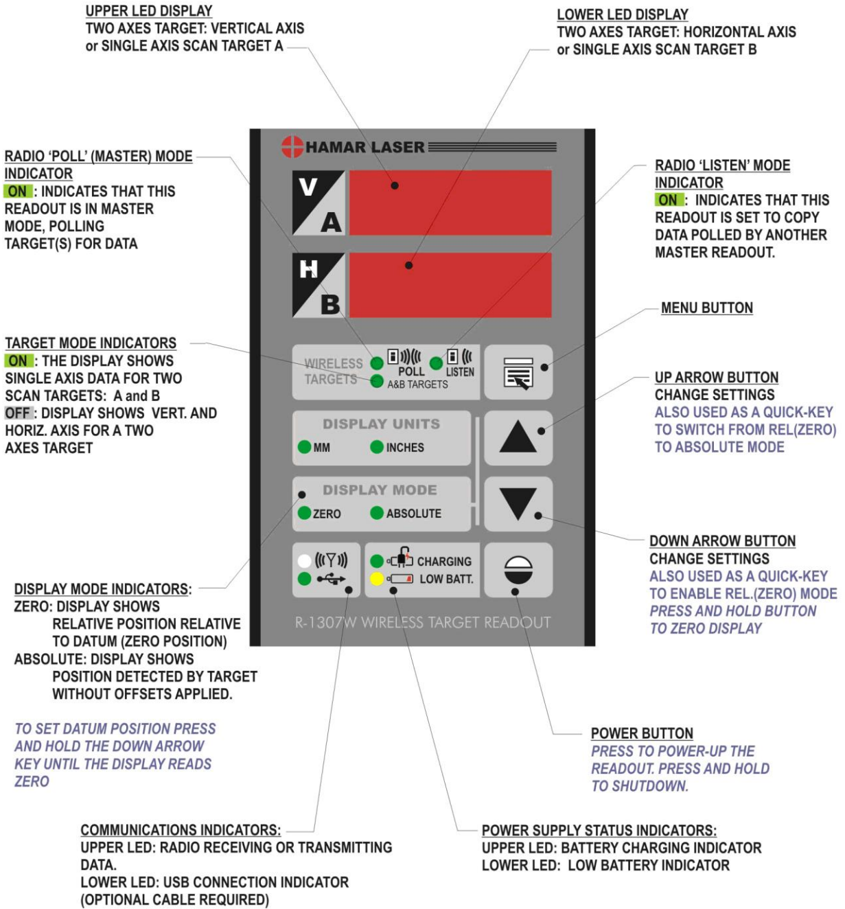
Figure 6 – R-1307W Readout Control Panel Features
