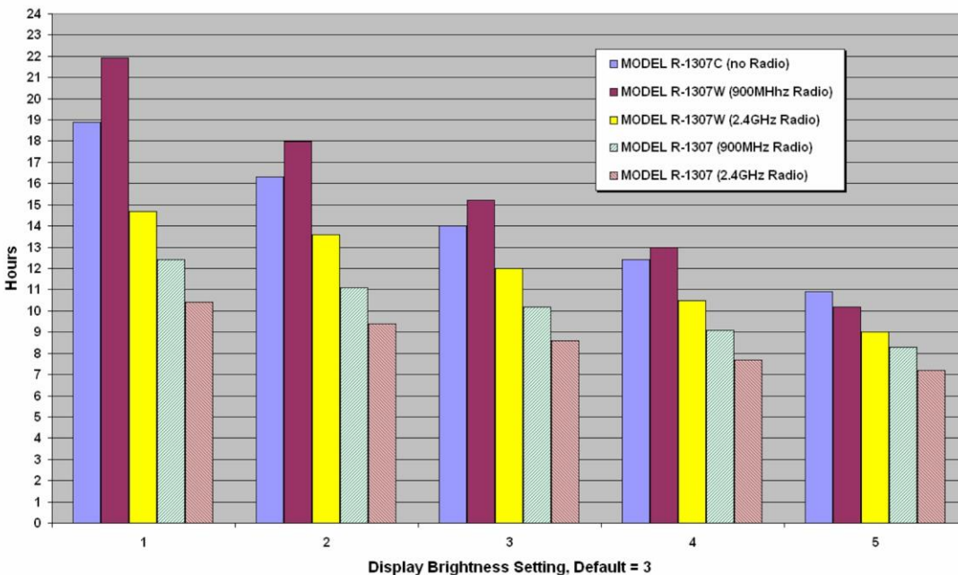
Battery Capacity vs. Display Brightness, All Models
