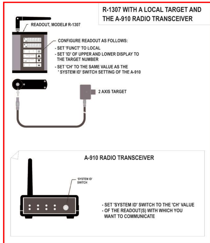
Figure 15— R-1307 with Cabled (Local) Target and A-910 Radio Transceiver
