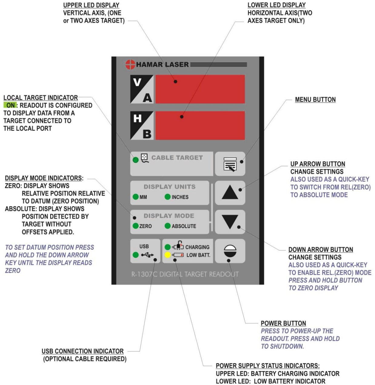
Figure 7 – R-1307C Readout Control Panel Features
