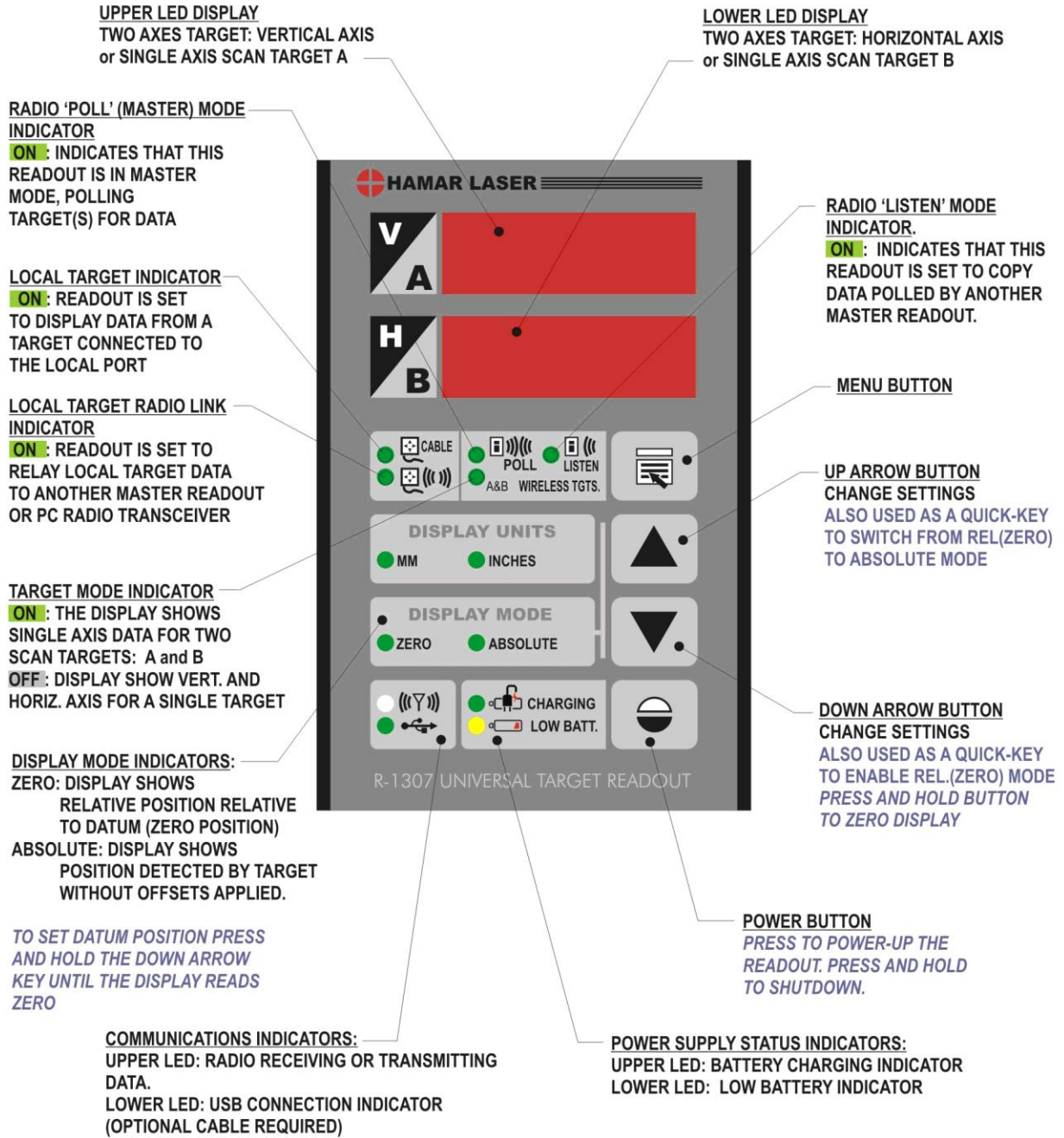
Figure 5 – R-1307 Models Control Panel Features
